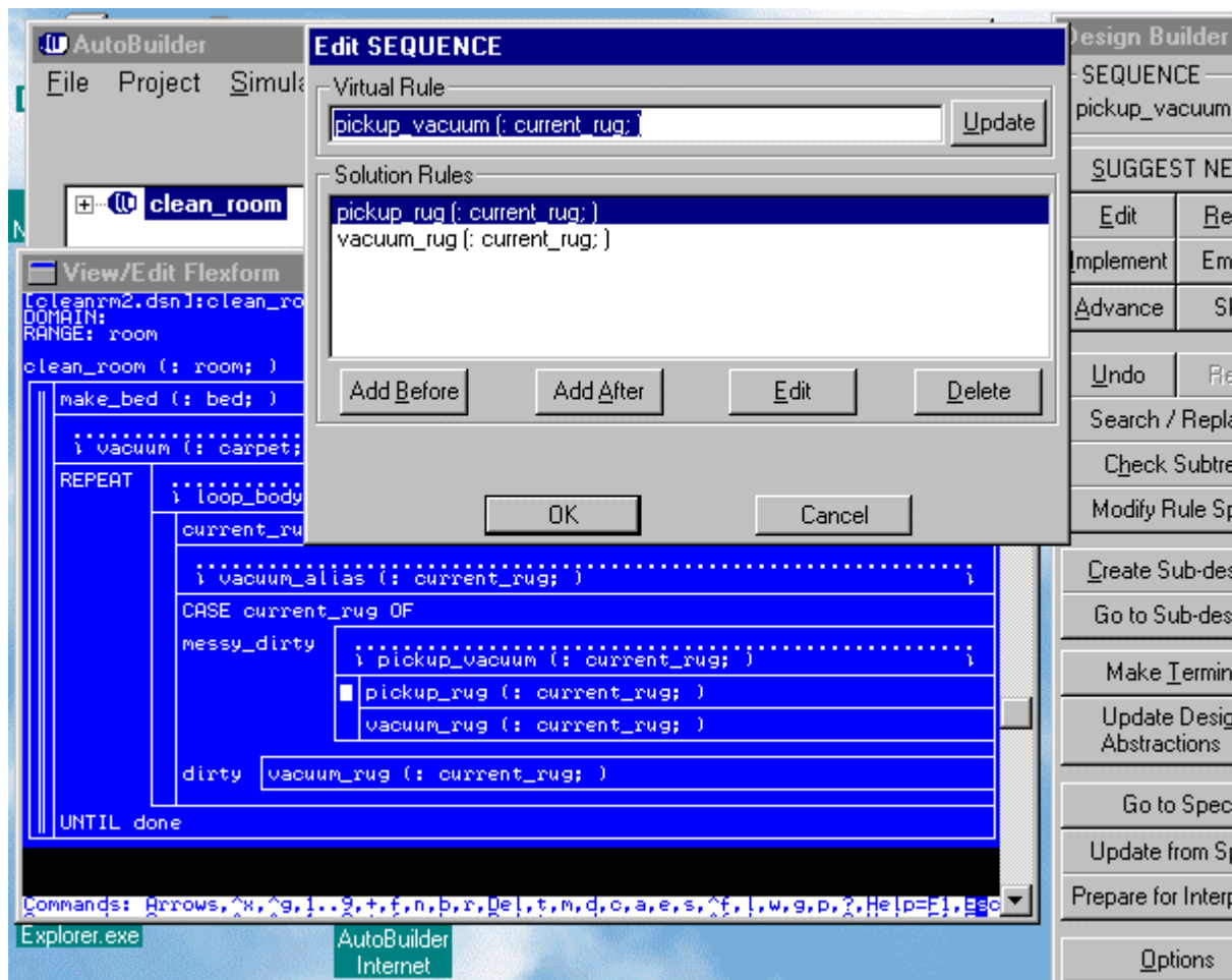
Figure 5. AutoBuilder in the process of refining the virtual component, pickup_vacuum (:current_rug;) , into a sequence.
