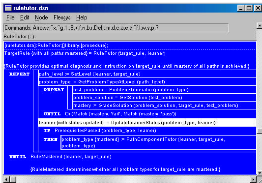
Figure 3. The General Purpose RuleTutor represented as a Flexform in Softbuilder.
