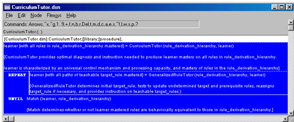
Figure 4. The General Purpose CurriculumTutor represented as a Flexform in Softbuilder.
